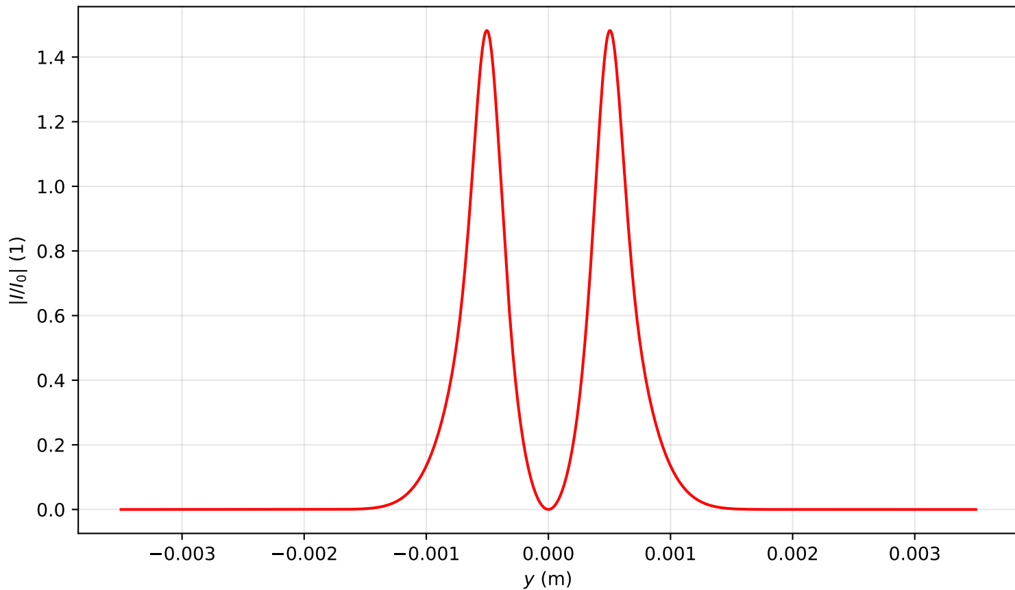
Intensity profile I(x=0, y, z=0.318)/I_0 , P_{in}=9.0P_{cr} , artificial time
